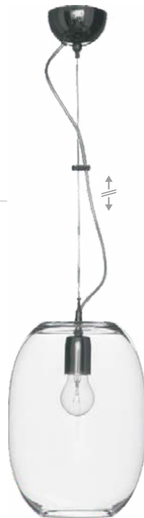
3594 IBIZA EGG ↑ 120 cm ↓ 30 cm ∅ 20 cm 1 x E27, max 60W
