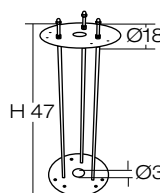
code 00A405.01P Anchor Bolt
