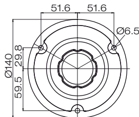
Cod. 00APR6 Anchor Bolt
