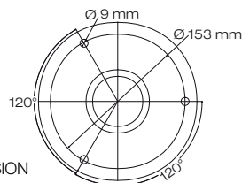
Anchor Bolt code 00APB
