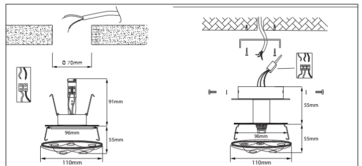
Einbau/recessed
