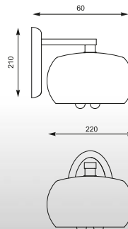
RAIN Wall W0076-01D-F4K9 1*G9 MAX 53W metal chrome / smoky glass / crystal drops inside IP20
